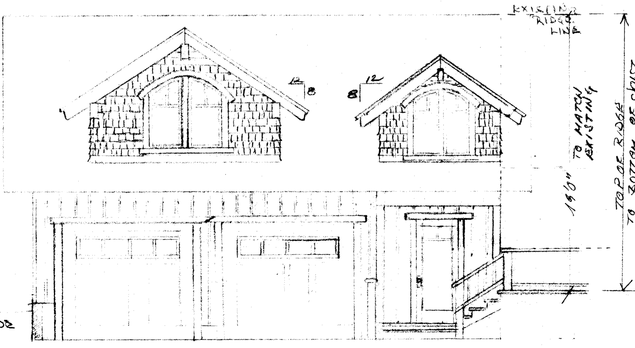
NORTH ELEVATION
