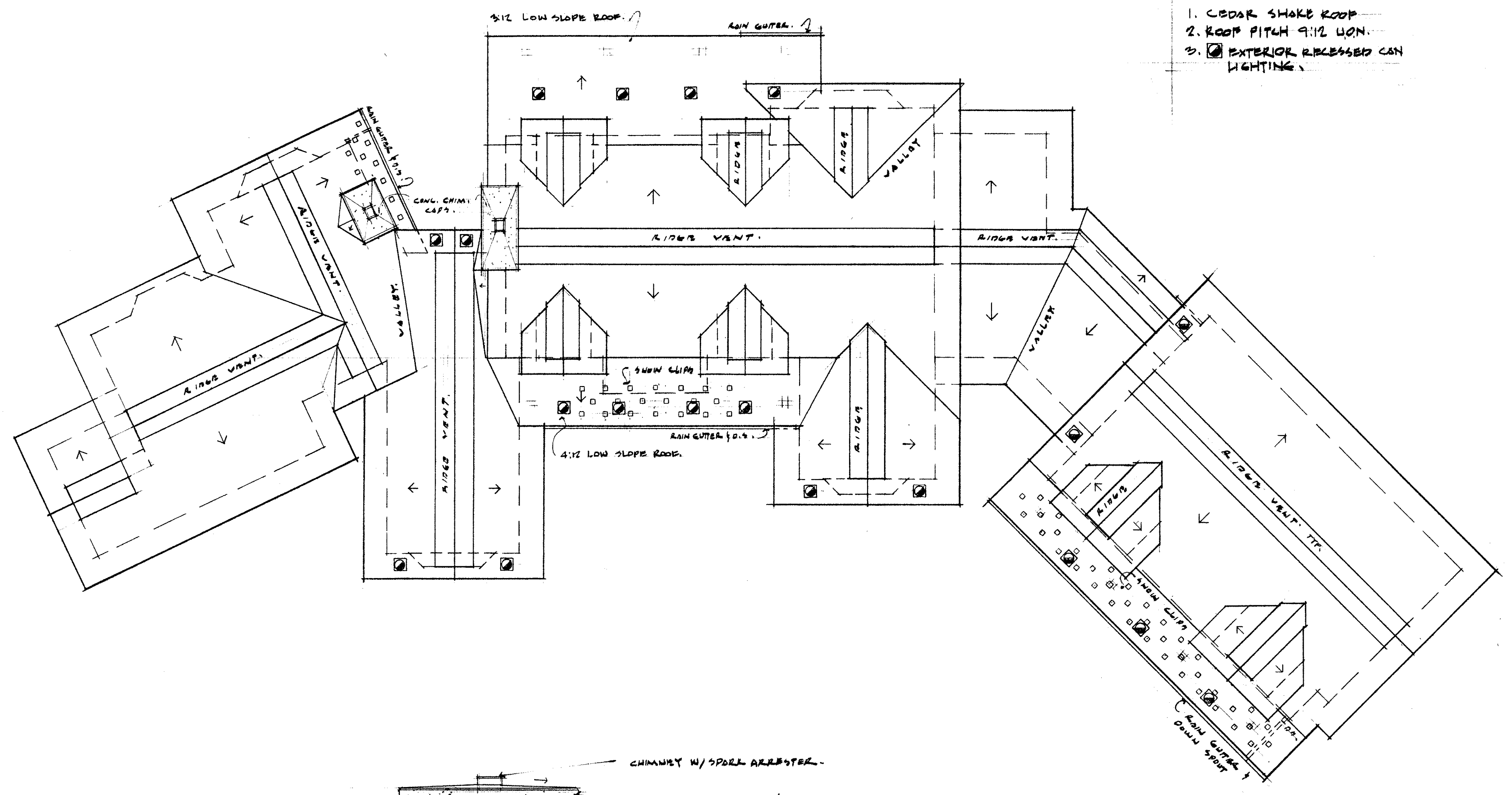
ROOF PLAN AND EXTERIOR LIGHTING
