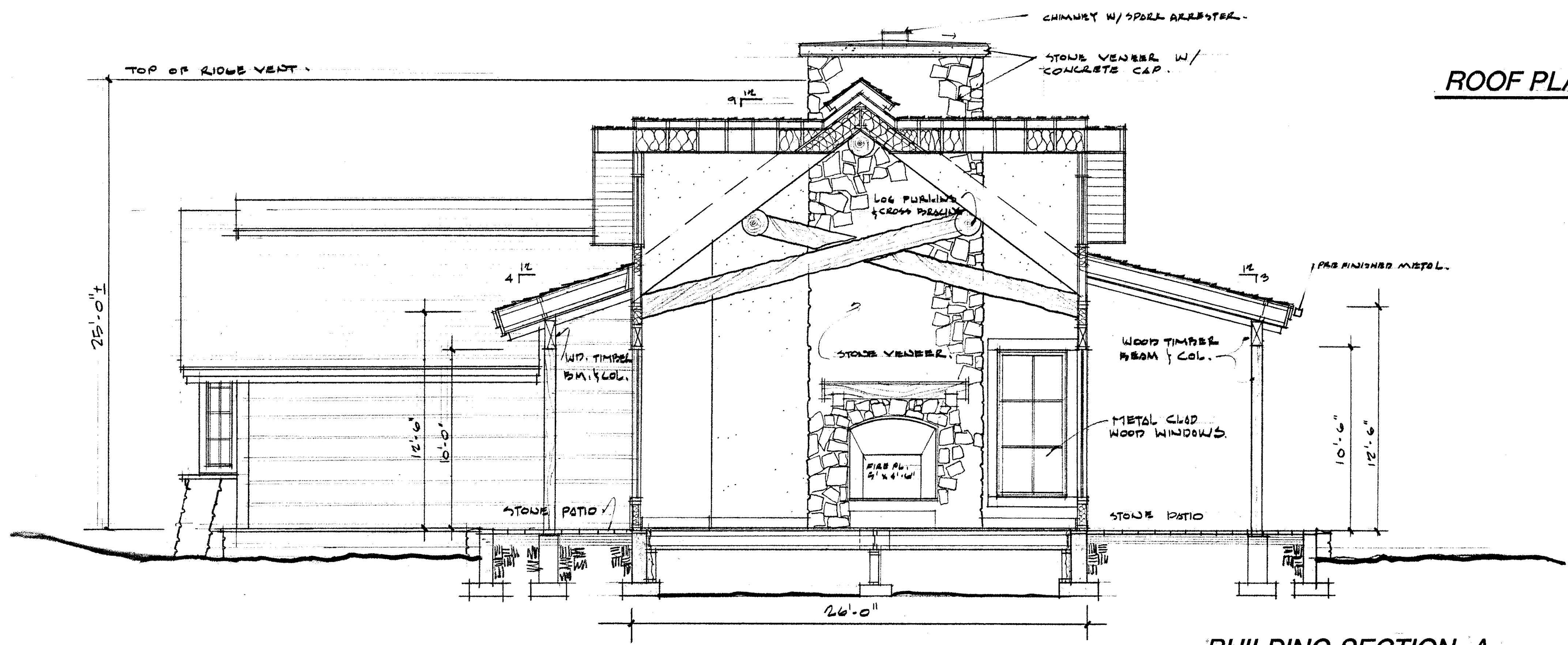
BUILDING SECTION A
